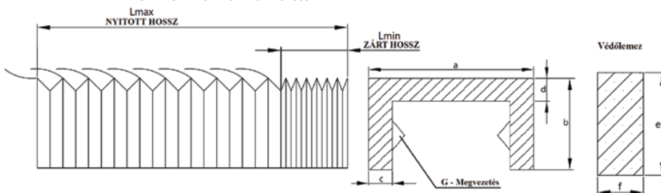
FBA/FBAm - FBG/FBGm harmonika méretei
