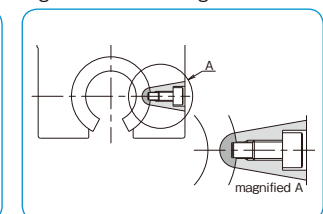
Figure D-8 Pin Fixing
